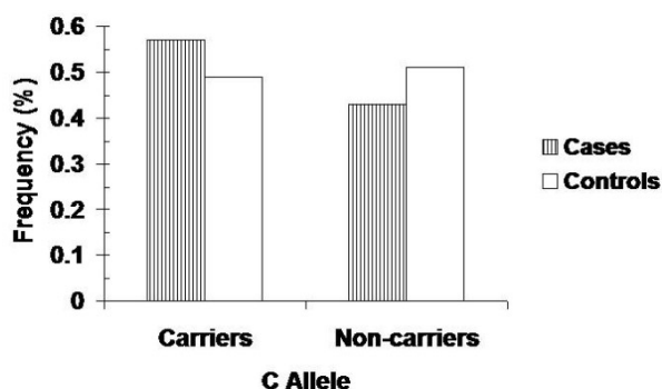
Figure 1. Prevalence of genotype frequencies by C allele carrier status, \chi^2=4.0 , df=1 , P=0.03
